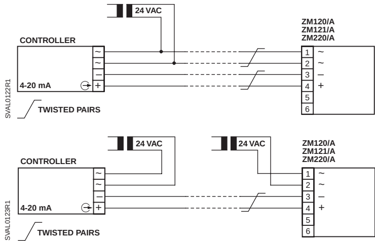
Figure 6. ZM../A with 4 – 20 mA Control Signal.
