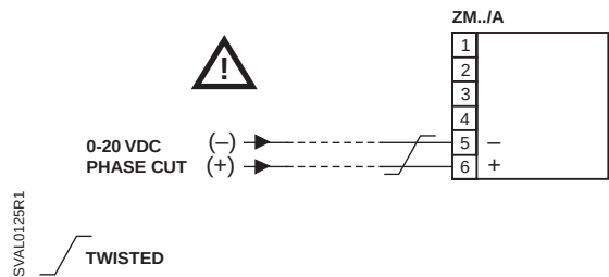
Figure 8. ZM100/A, ZM101/A, ZM200/A, ZM120/A, ZM121/A, ZM220/A (With Power Amplifier).
