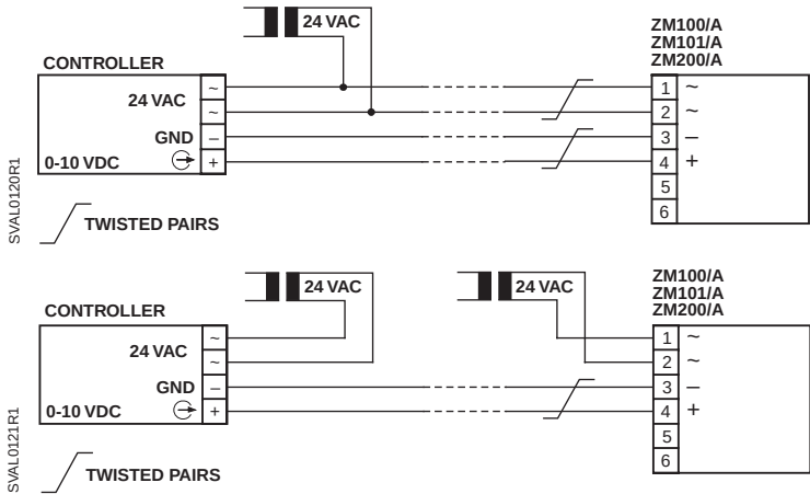
Figure 5. Four-wire Connection to Controller.
